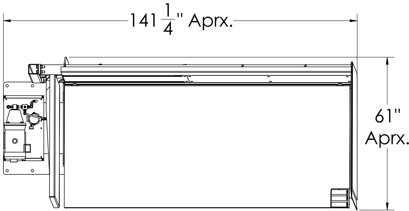
Shipping Position
