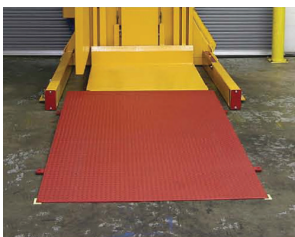
LOADING RAMP: Heavy-duty reinforced ramp which allows for manual and electric pallet truck entry
